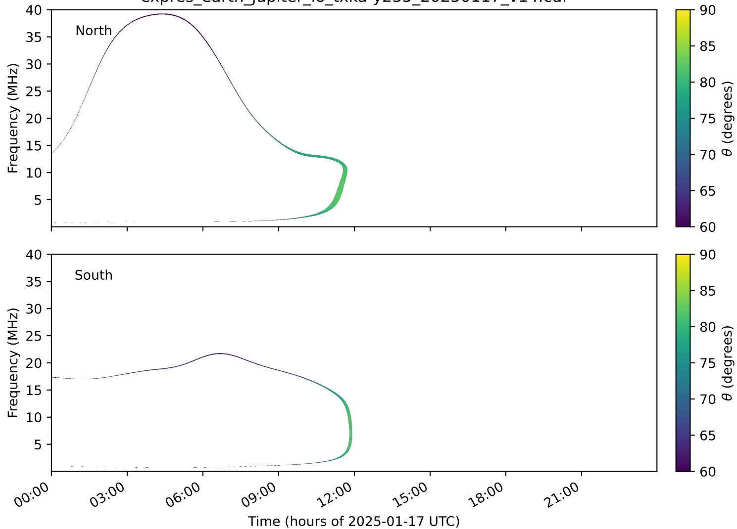
expres_earth_jupiter_io_txka-y235_20250117_v14.cdf
