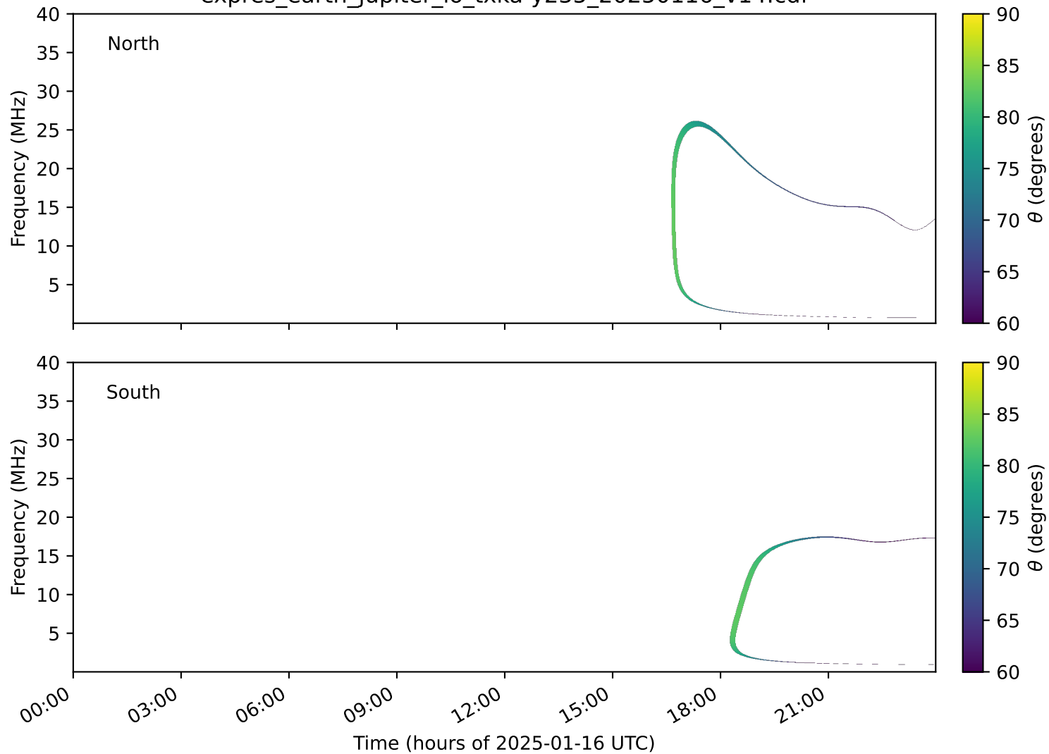
expres_earth_jupiter_io_txka-y235_20250116_v14.cdf
