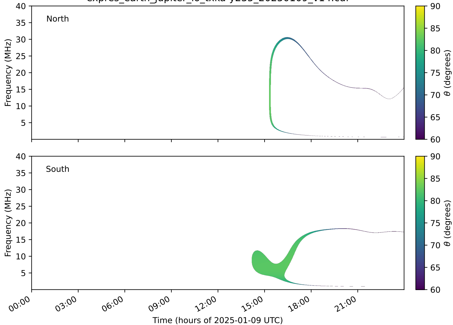
expres_earth_jupiter_io_txka-y235_20250109_v14.cdf
