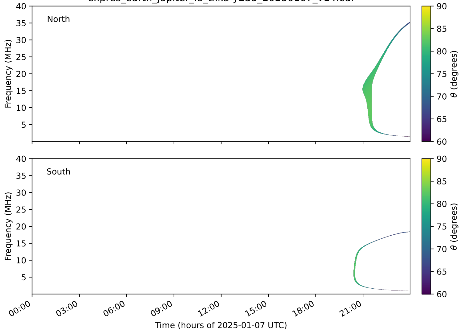
expres_earth_jupiter_io_txka-y235_20250107_v14.cdf
