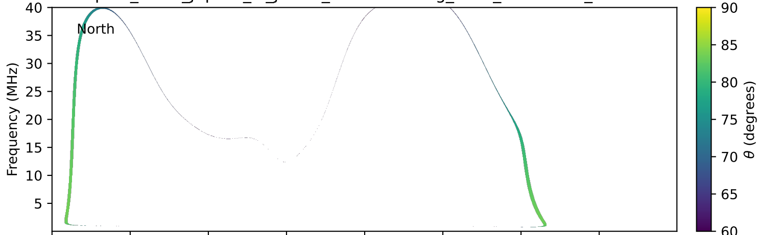
expres_earth_jupiter_io_jrm33_lossc-wid1deg_3kev_20250122_v11.cdf
