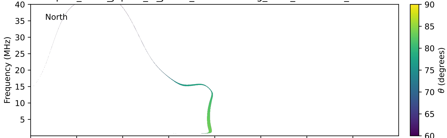
expres_earth_jupiter_io_jrm33_lossc-wid1deg_3kev_20250117_v11.cdf
