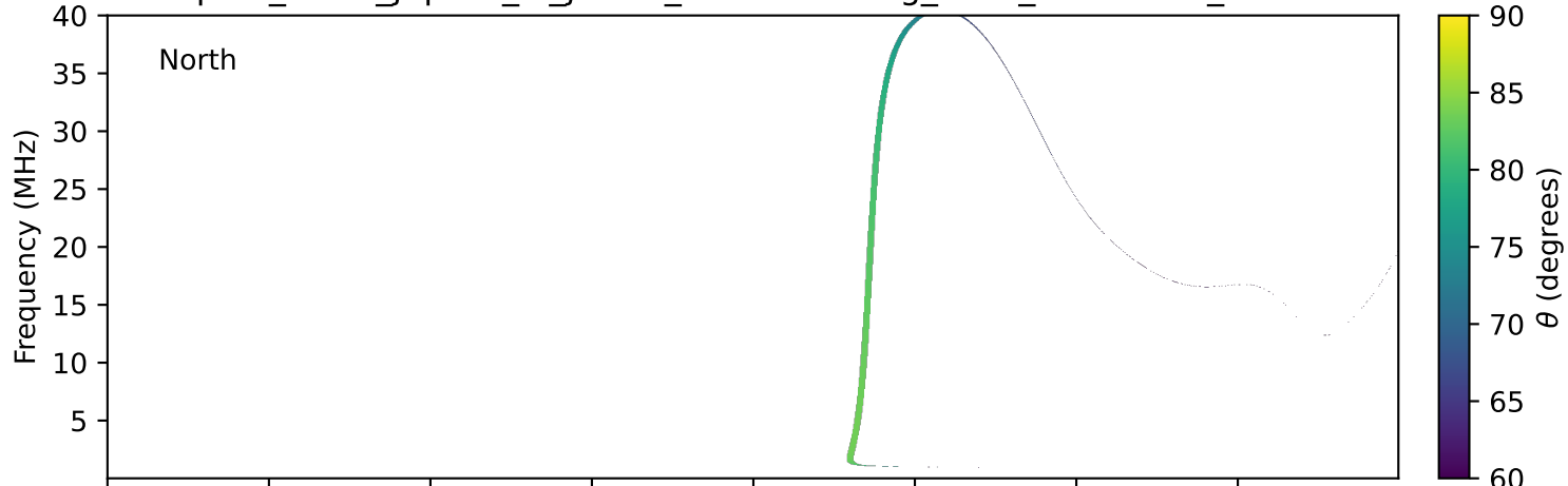
expres_earth_jupiter_io_jrm33_lossc-wid1deg_3kev_20250102_v11.cdf
