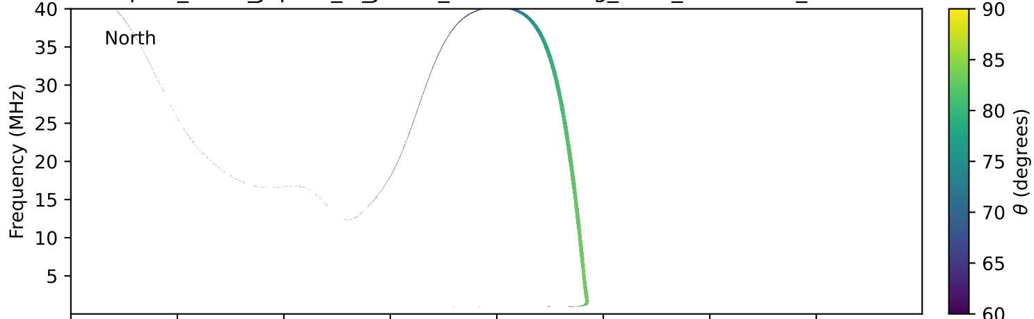
expres_earth_jupiter_io_jrm33_lossc-wid1deg_3kev_20250101_v11.cdf
