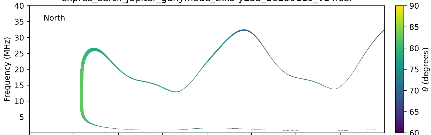
expres_earth_jupiter_ganymede_txka-y235_20250119_v14.cdf
