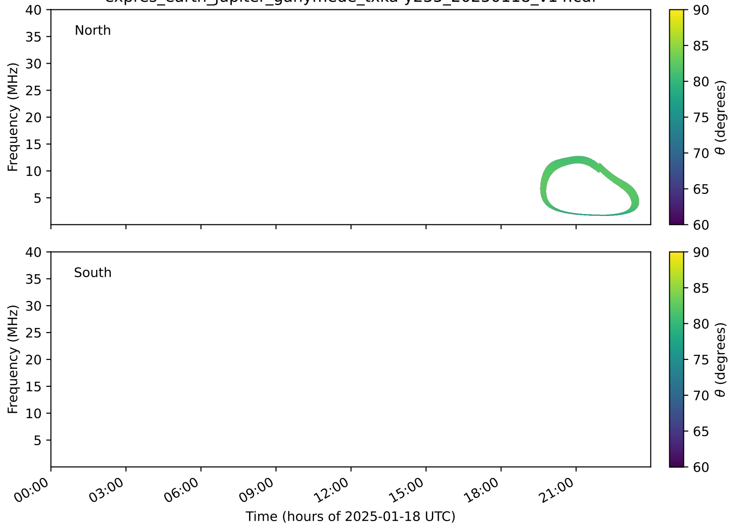
expres_earth_jupiter_ganymede_txka-y235_20250118_v14.cdf
