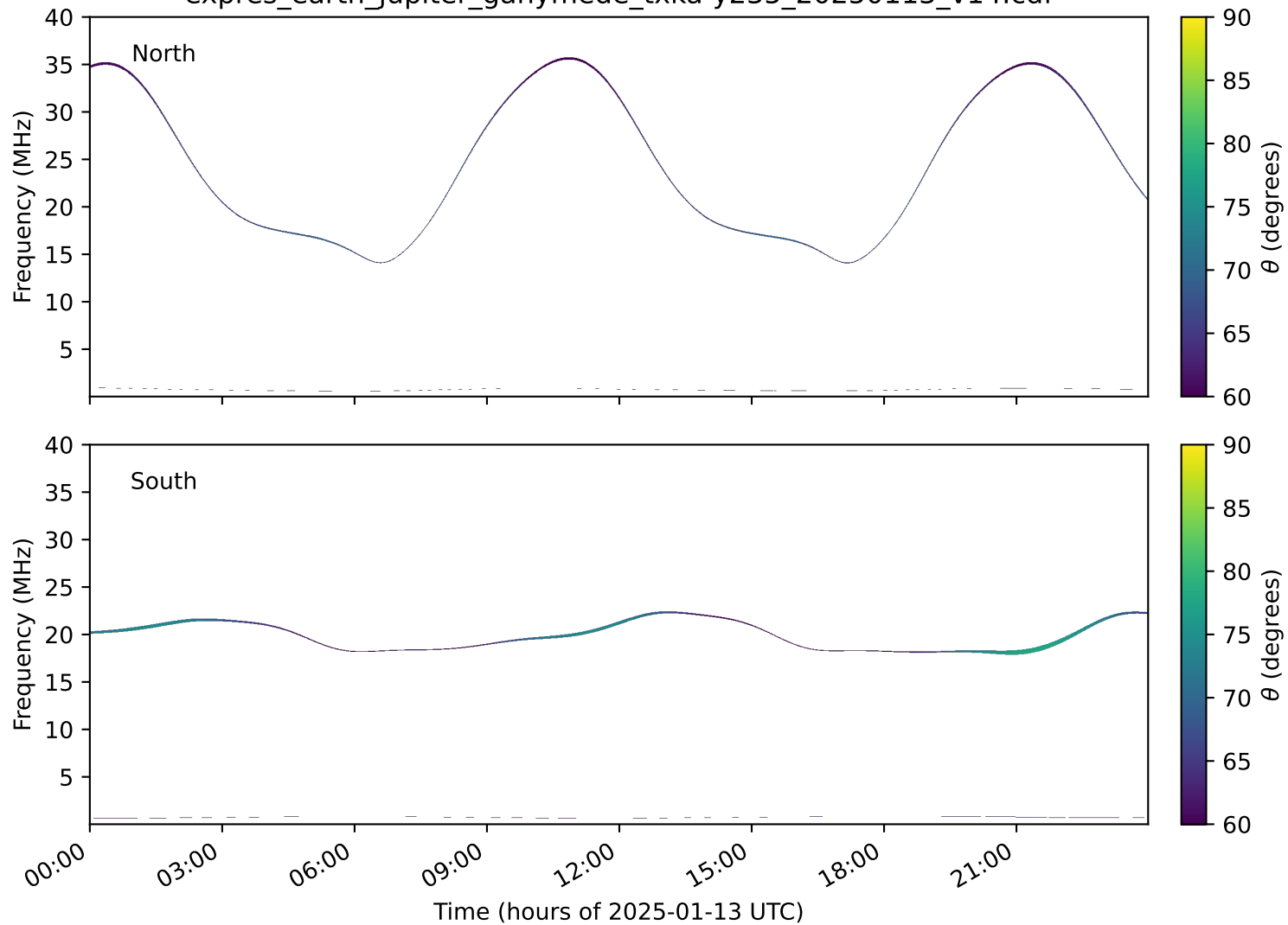
expres_earth_jupiter_ganymede_txka-y235_20250113_v14.cdf
