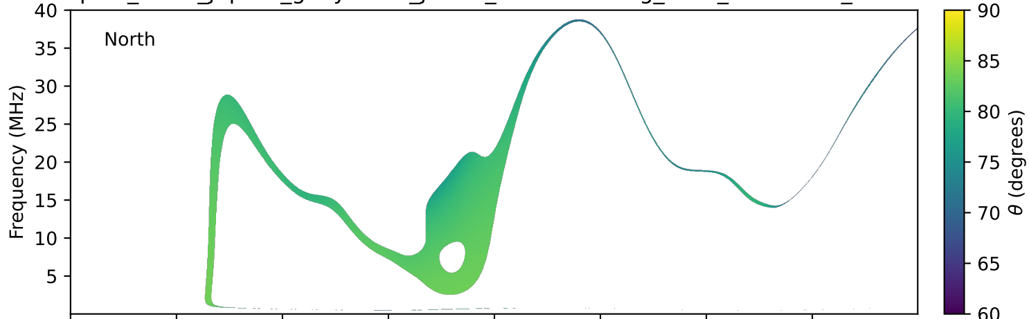
expres_earth_jupiter_ganymede_jrm33_lossc-wid1deg_3kev_20250119_v11.cdf
