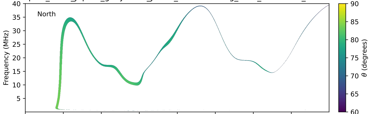
expres_earth_jupiter_ganymede_jrm33_lossc-wid1deg_3kev_20250112_v11.cdf
