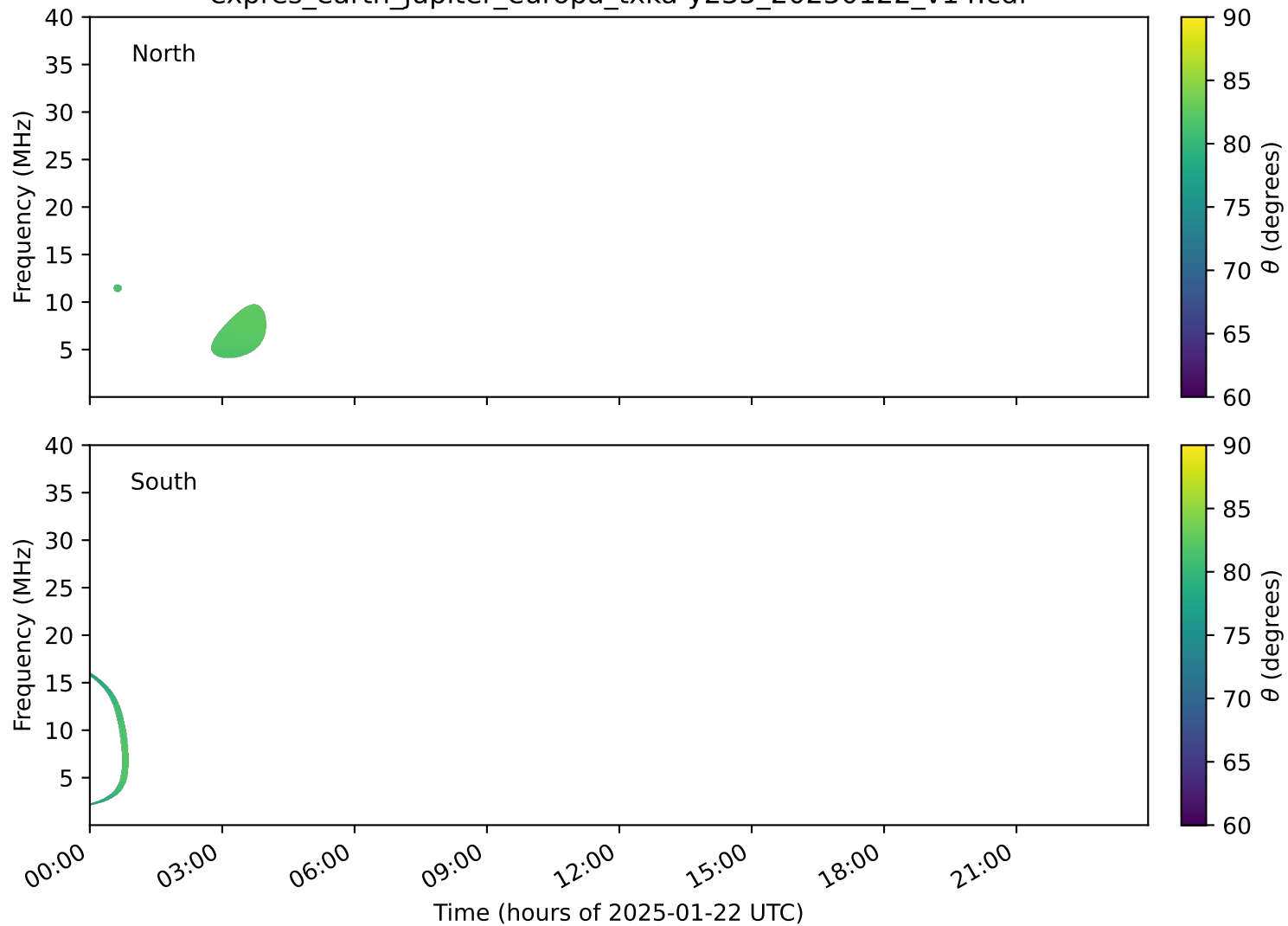
expres_earth_jupiter_europa_txka-y235_20250122_v14.cdf
