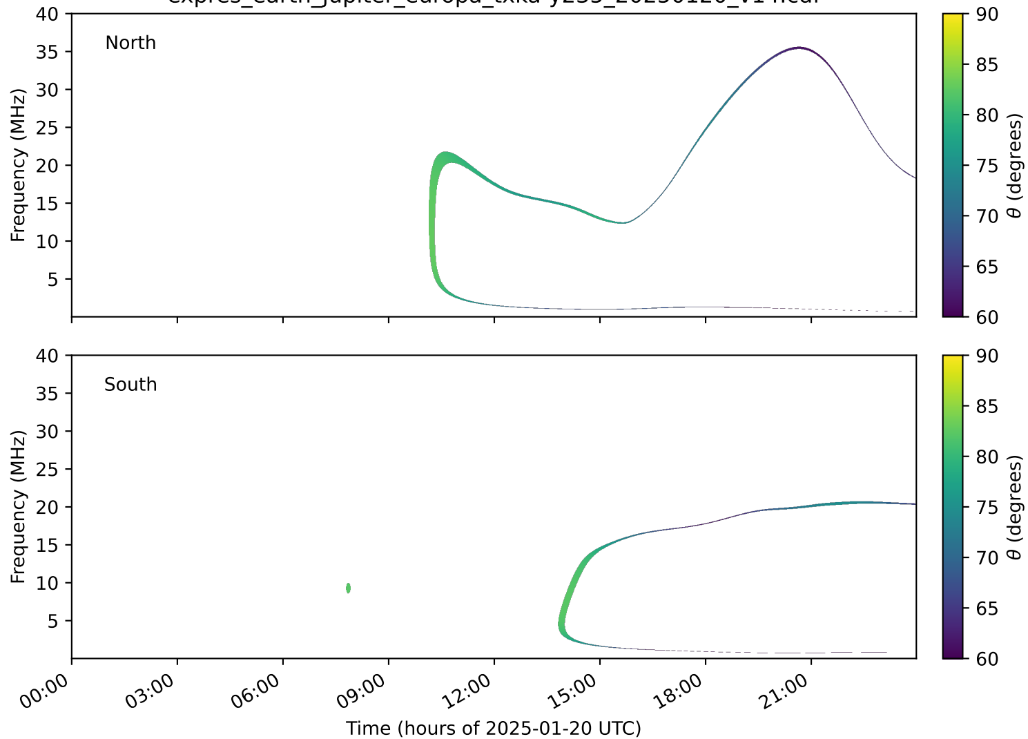
expres_earth_jupiter_europa_txka-y235_20250120_v14.cdf
