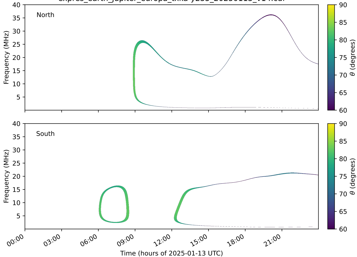
expres_earth_jupiter_europa_txka-y235_20250113_v14.cdf
