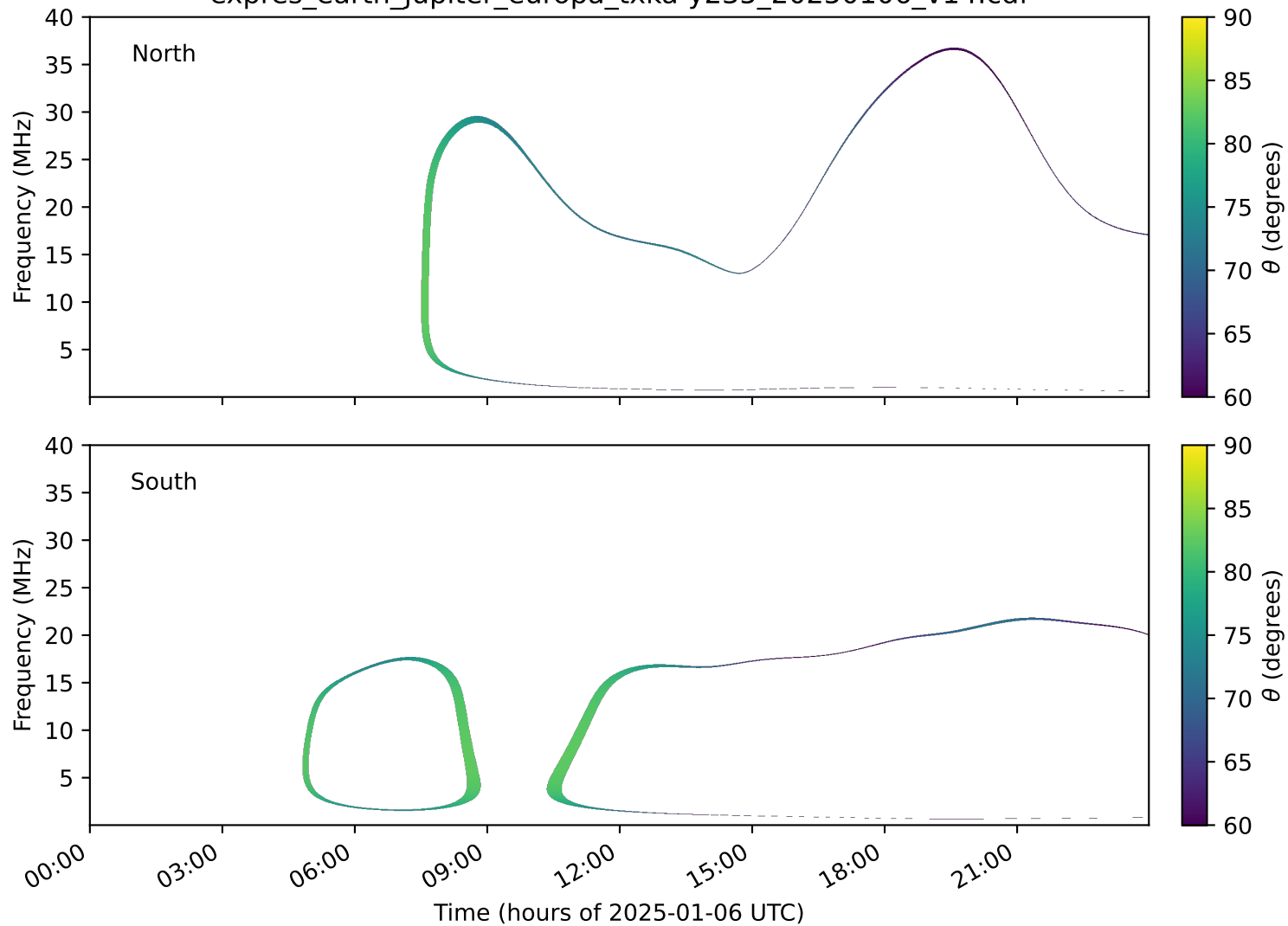
expres_earth_jupiter_europa_txka-y235_20250106_v14.cdf
