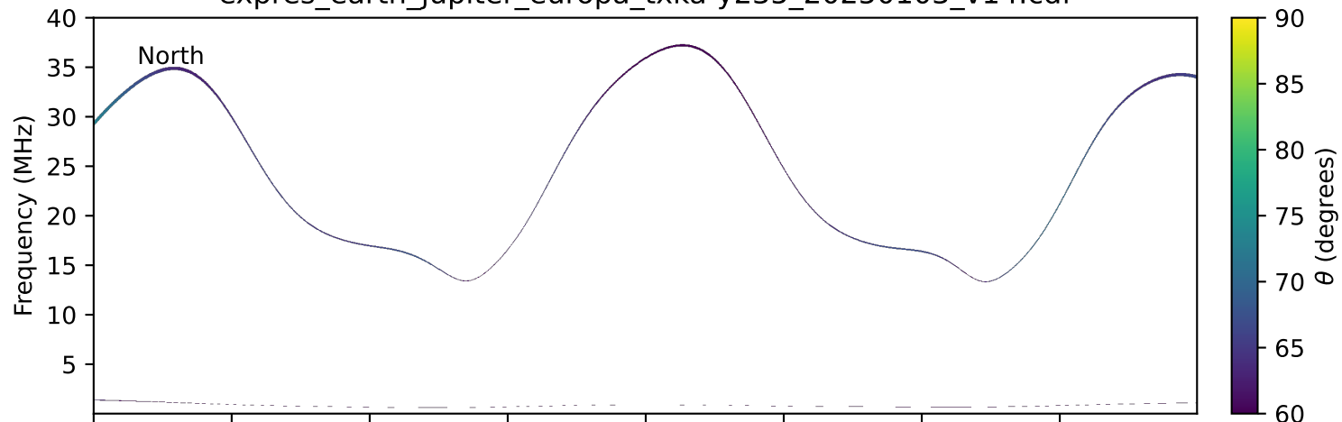
expres_earth_jupiter_europa_txka-y235_20250103_v14.cdf
