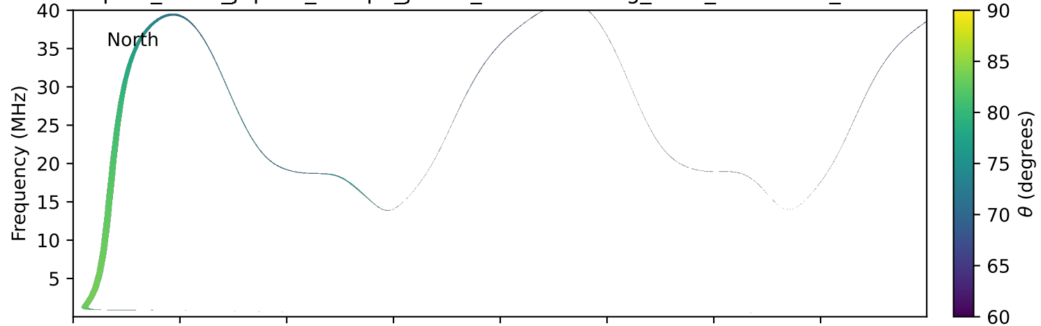
expres_earth_jupiter_europa_jrm33_lossc-wid1deg_3kev_20250117_v11.cdf
