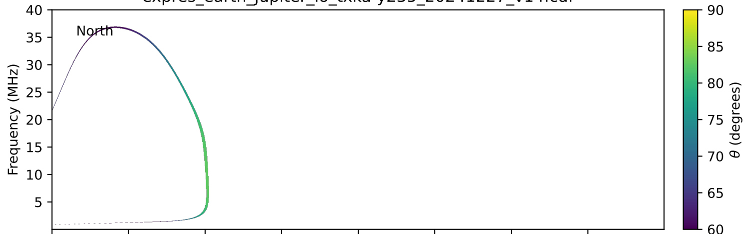
expres_earth_jupiter_io_txka-y235_20241227_v14.cdf
