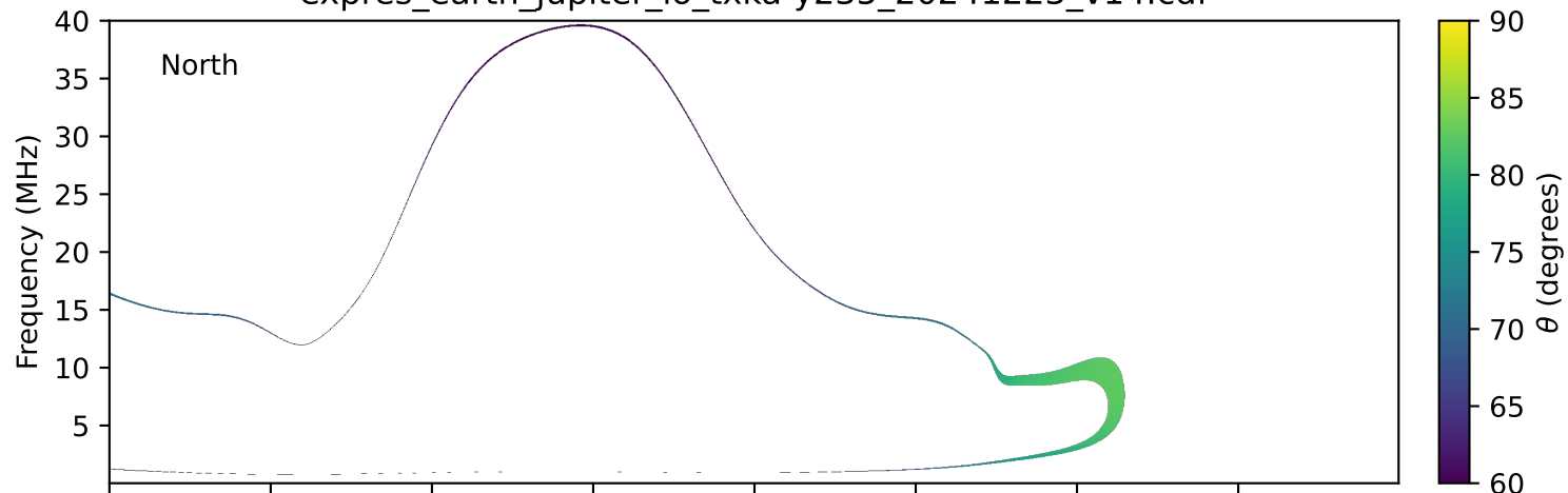
expres_earth_jupiter_io_txka-y235_20241223_v14.cdf
