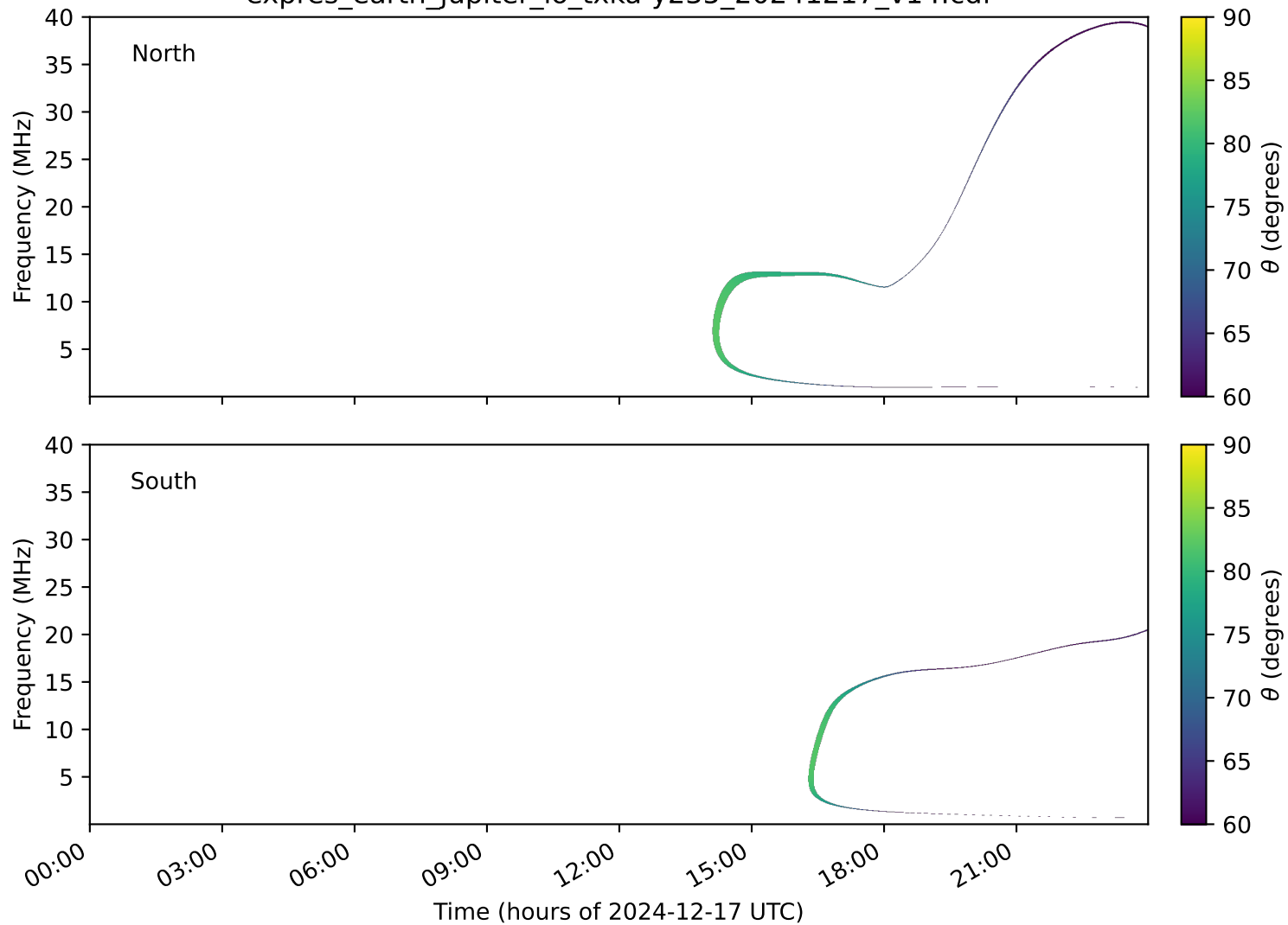
expres_earth_jupiter_io_txka-y235_20241217_v14.cdf
