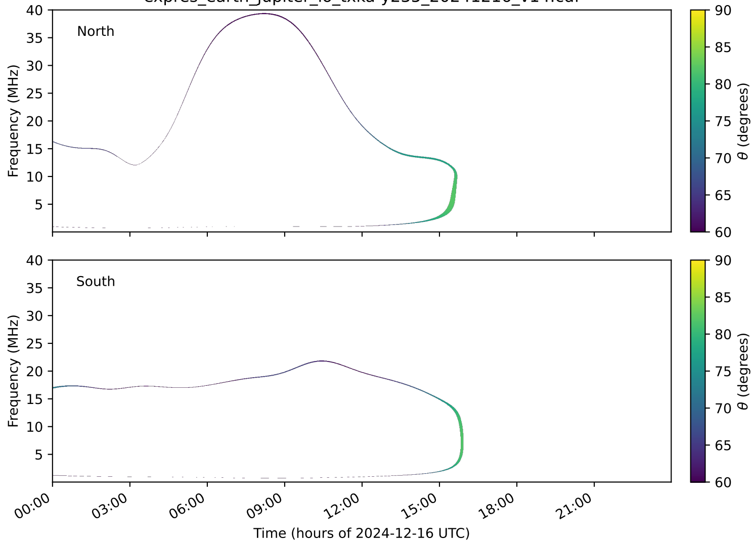
expres_earth_jupiter_io_txka-y235_20241216_v14.cdf
