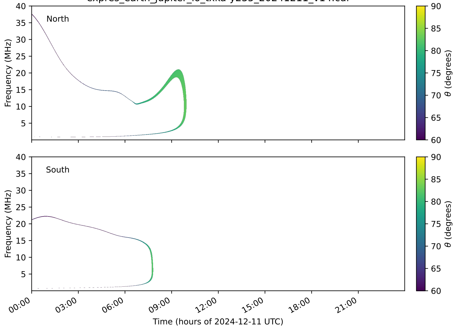
expres_earth_jupiter_io_txka-y235_20241211_v14.cdf
