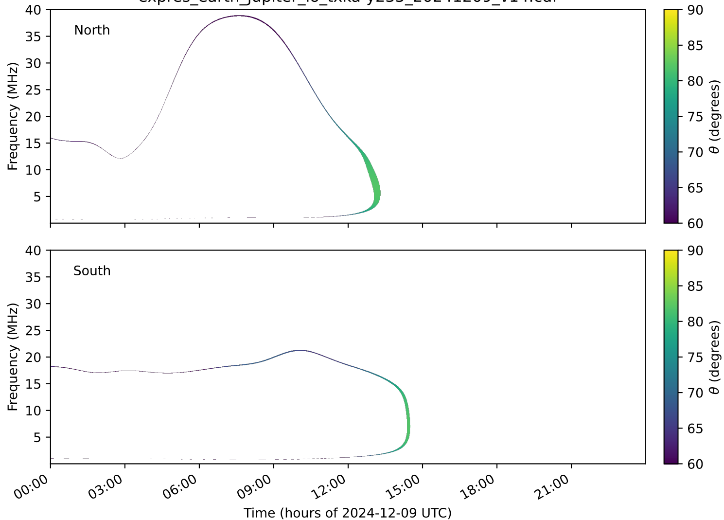
expres_earth_jupiter_io_txka-y235_20241209_v14.cdf
