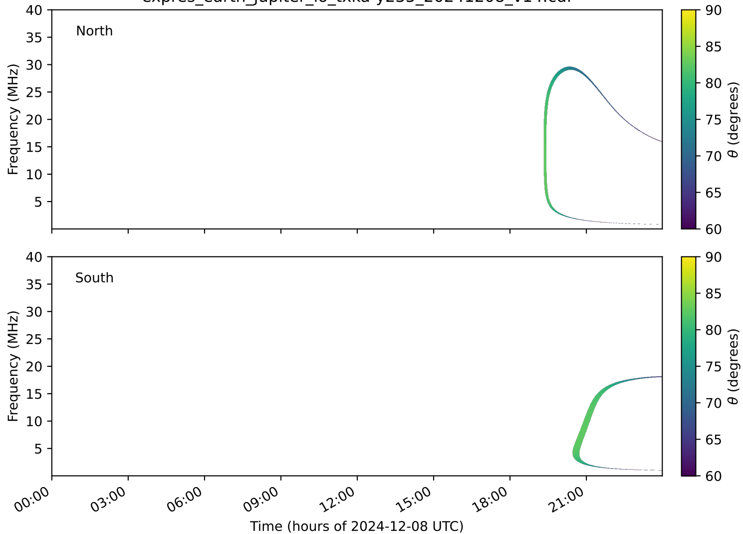
expres_earth_jupiter_io_txka-y235_20241208_v14.cdf
