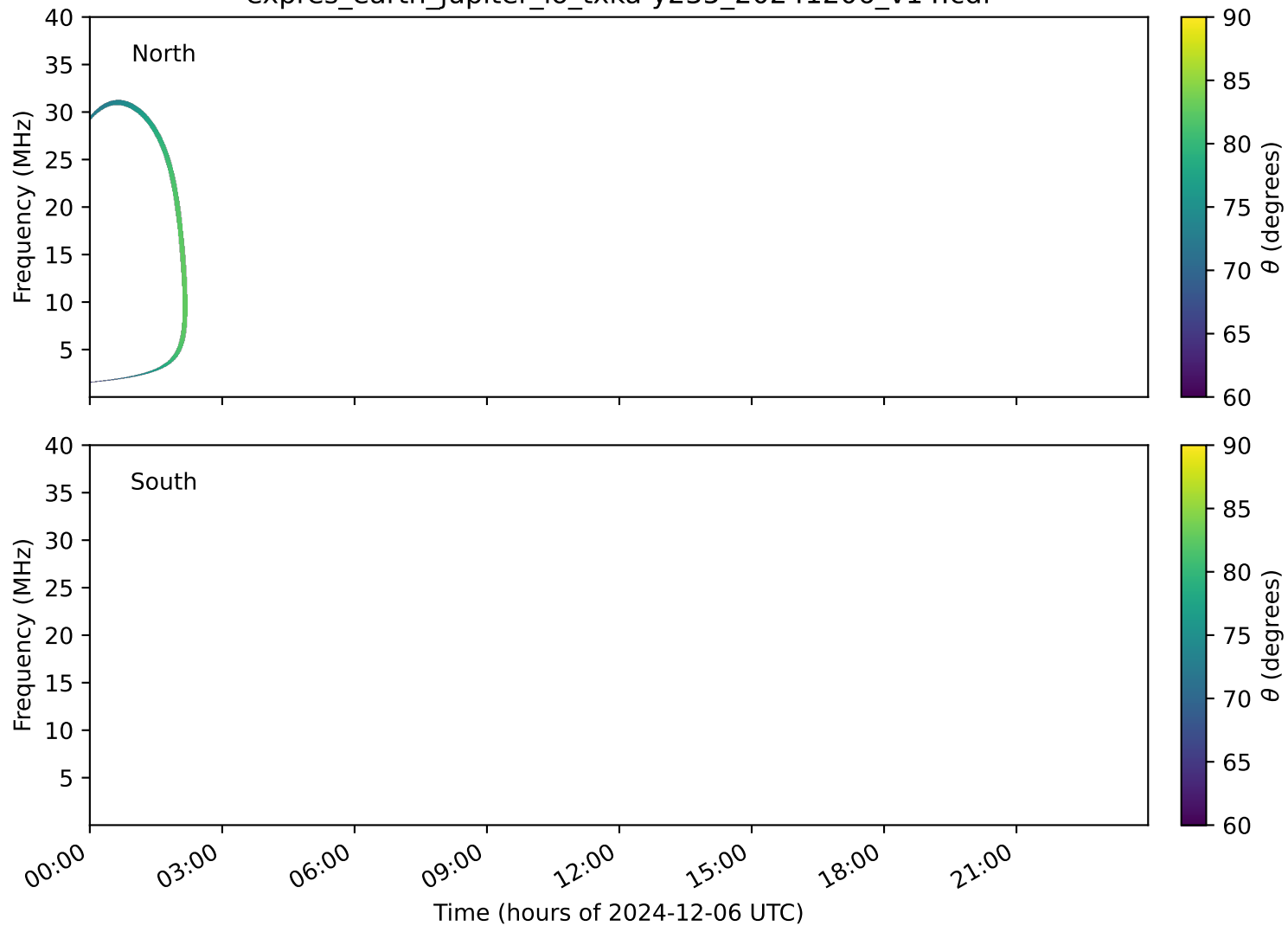
expres_earth_jupiter_io_txka-y235_20241206_v14.cdf
