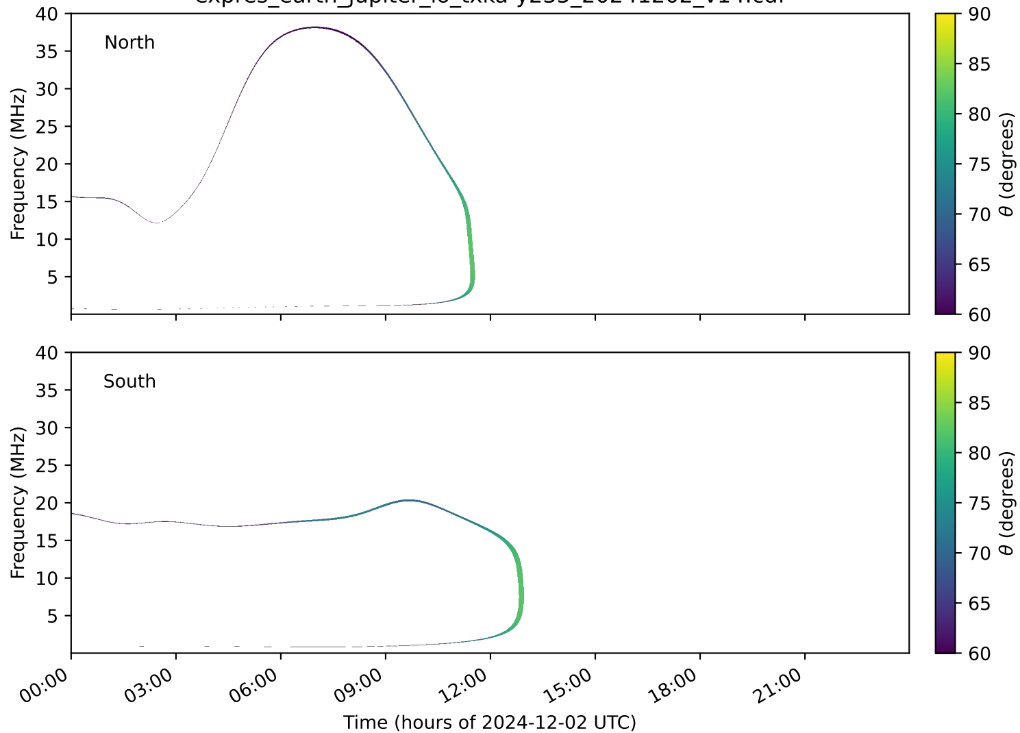
expres_earth_jupiter_io_txka-y235_20241202_v14.cdf
