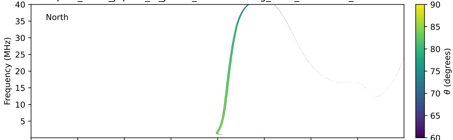
expres_earth_jupiter_io_jrm33_lossc-wid1deg_3kev_20241226_v11.cdf
