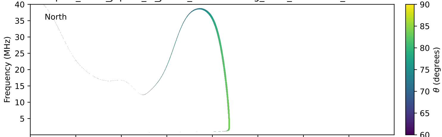
expres_earth_jupiter_io_jrm33_lossc-wid1deg_3kev_20241225_v11.cdf
