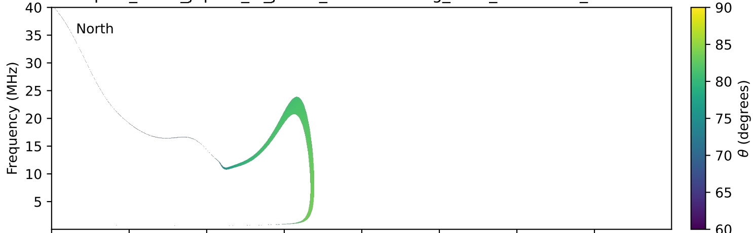
expres_earth_jupiter_io_jrm33_lossc-wid1deg_3kev_20241211_v11.cdf
