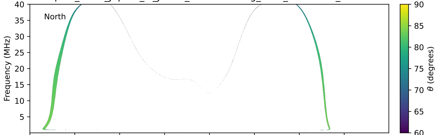
expres_earth_jupiter_io_jrm33_lossc-wid1deg_3kev_20241207_v11.cdf
