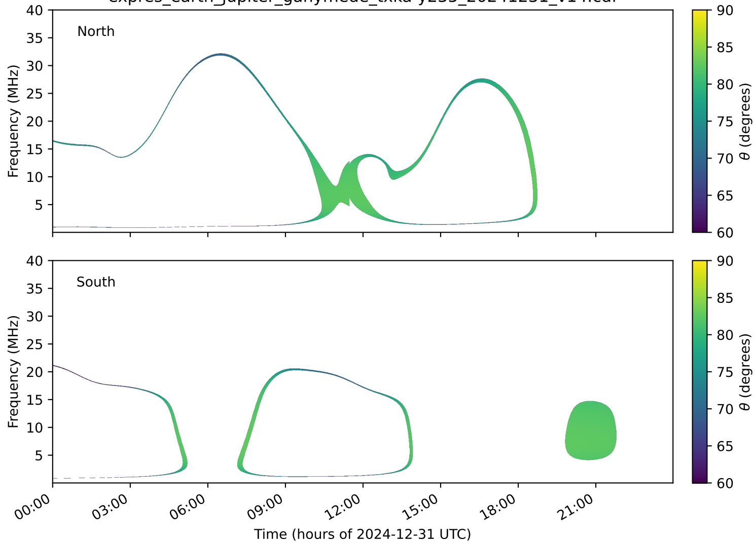
expres_earth_jupiter_ganymede_txka-y235_20241231_v14.cdf
