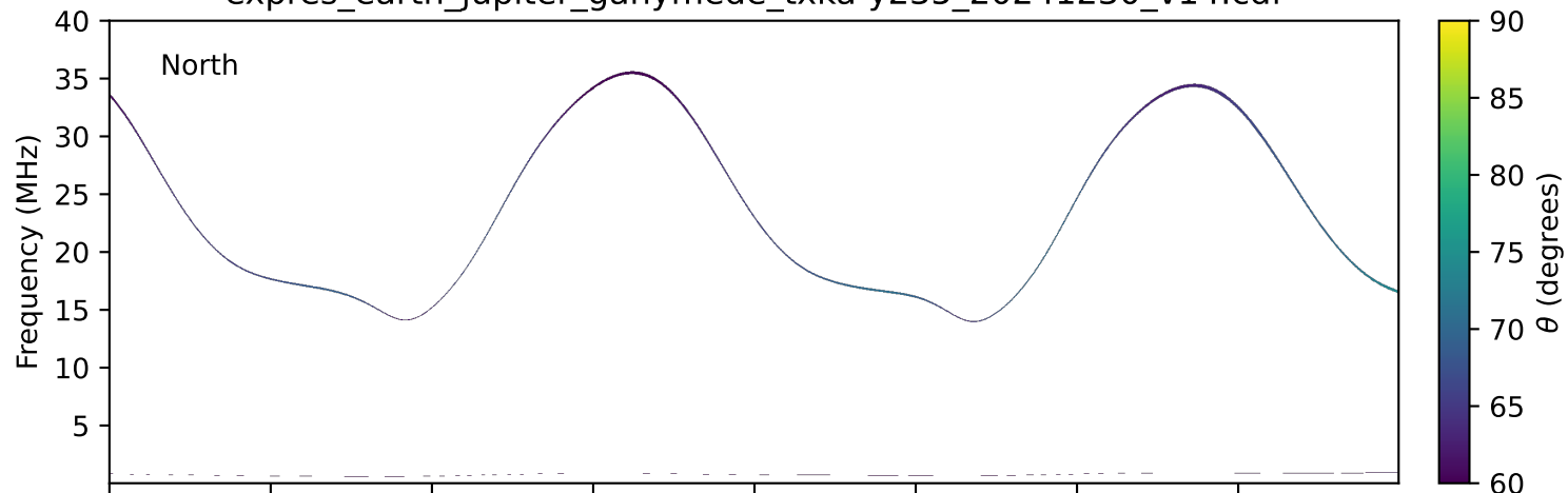
expres_earth_jupiter_ganymede_txka-y235_20241230_v14.cdf
