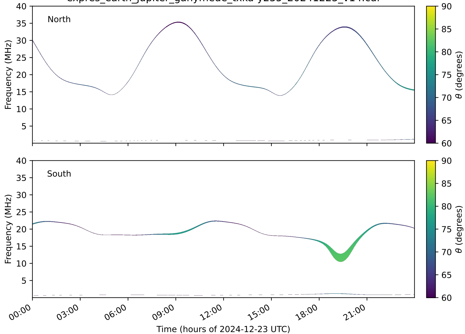
expres_earth_jupiter_ganymede_txka-y235_20241223_v14.cdf
