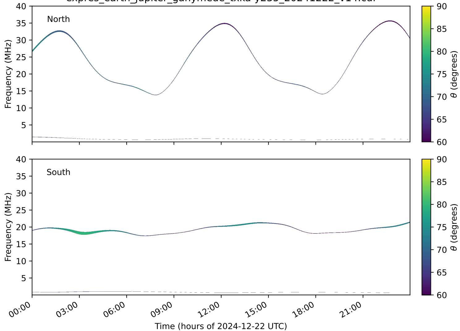
expres_earth_jupiter_ganymede_txka-y235_20241222_v14.cdf
