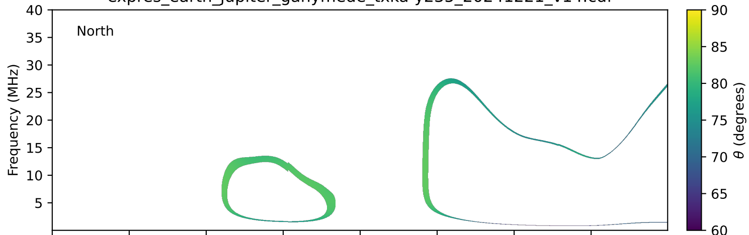
expres_earth_jupiter_ganymede_txka-y235_20241221_v14.cdf
