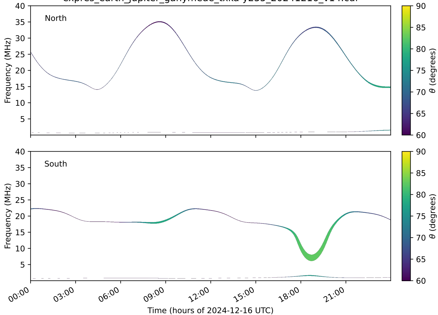
expres_earth_jupiter_ganymede_txka-y235_20241216_v14.cdf
