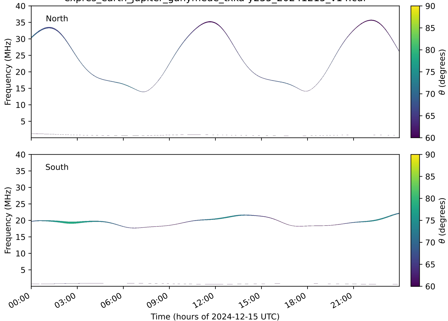
expres_earth_jupiter_ganymede_txka-y235_20241215_v14.cdf
