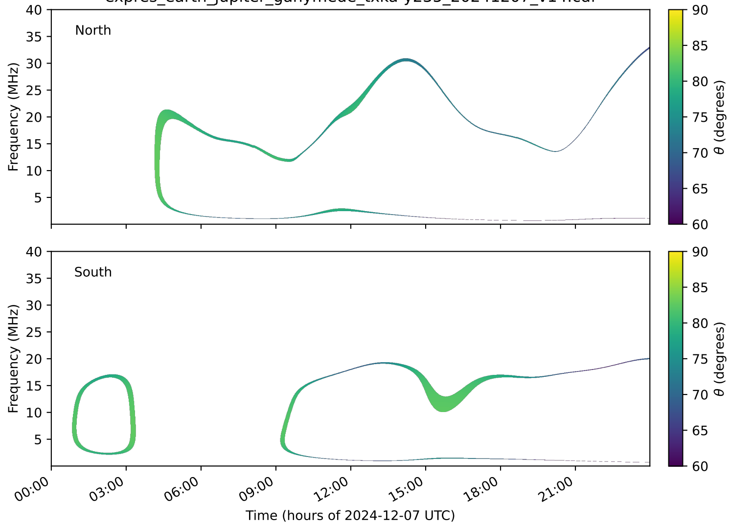
expres_earth_jupiter_ganymede_txka-y235_20241207_v14.cdf
