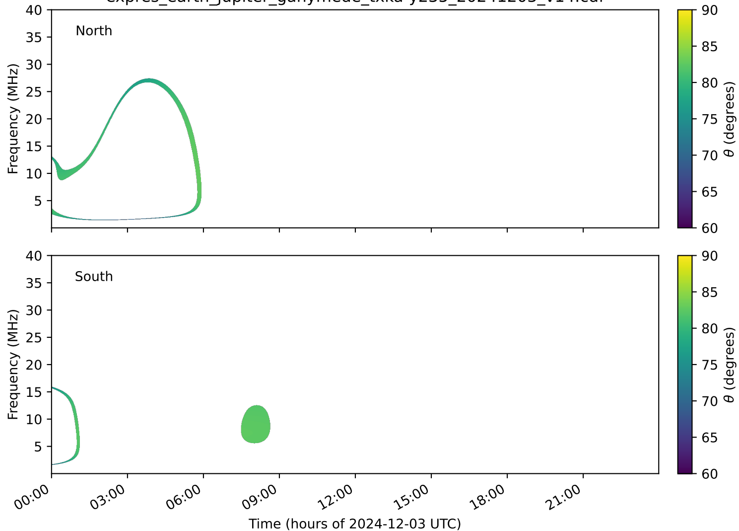
expres_earth_jupiter_ganymede_txka-y235_20241203_v14.cdf
