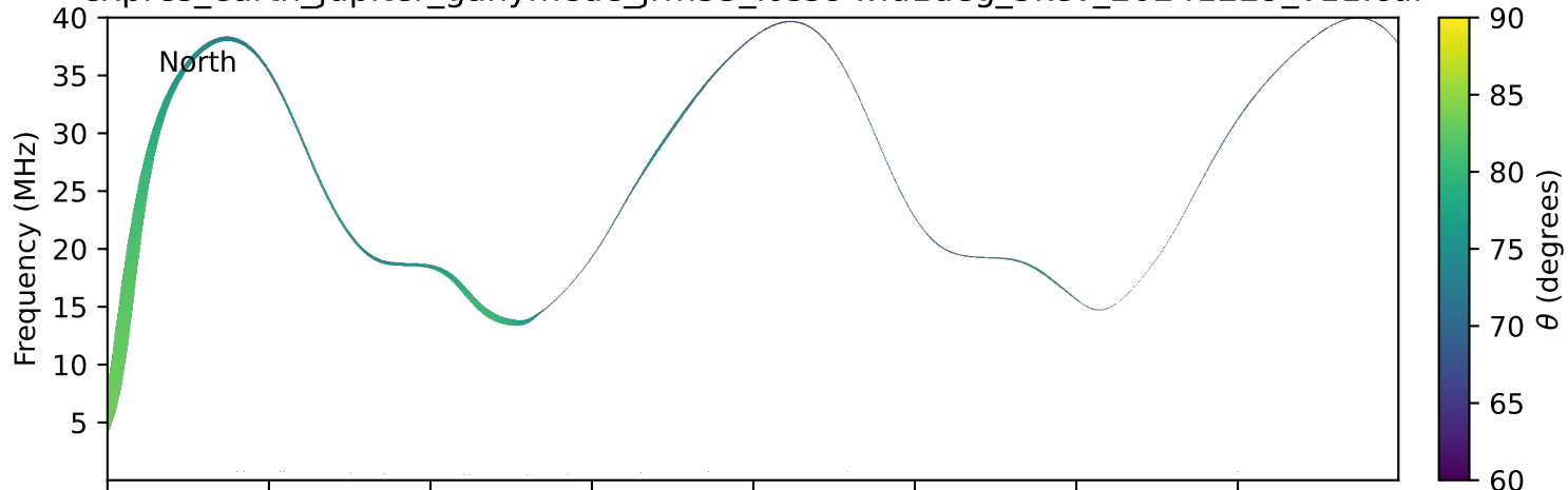
expres_earth_jupiter_ganymede_jrm33_lossc-wid1deg_3kev_20241229_v11.cdf
