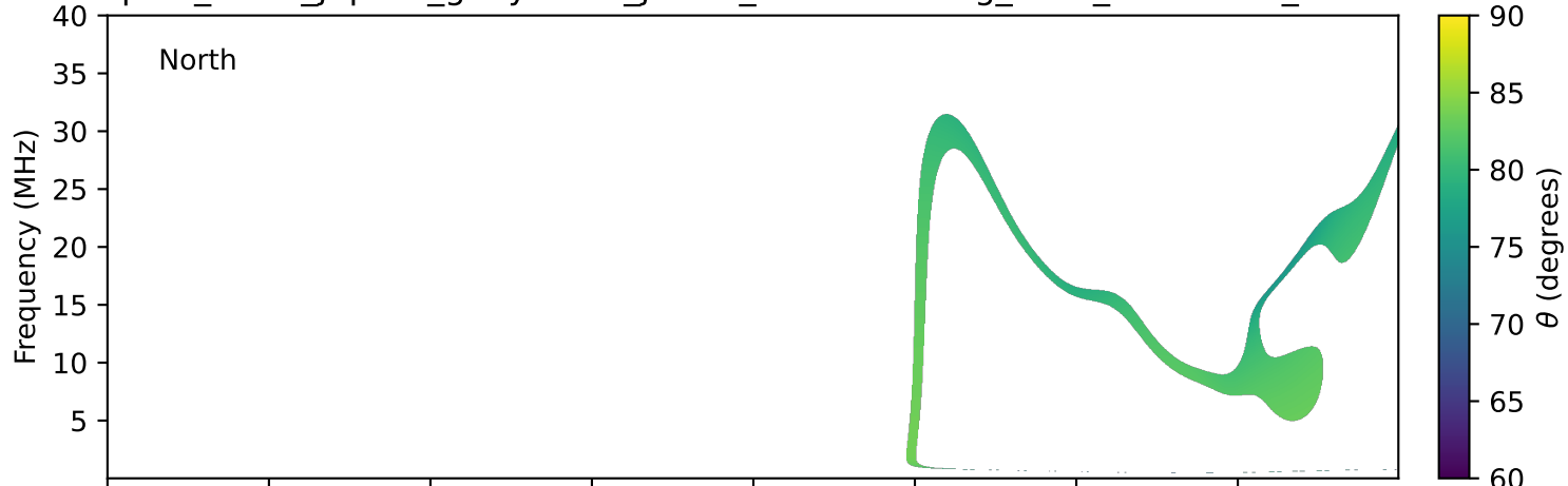
expres_earth_jupiter_ganymede_jrm33_lossc-wid1deg_3kev_20241221_v11.cdf
