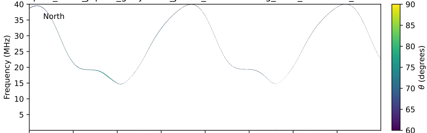
expres_earth_jupiter_ganymede_jrm33_lossc-wid1deg_3kev_20241208_v11.cdf
