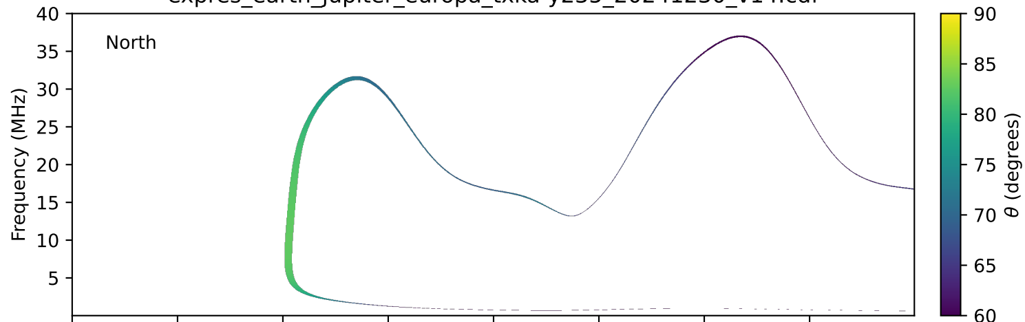
expres_earth_jupiter_europa_txka-y235_20241230_v14.cdf
