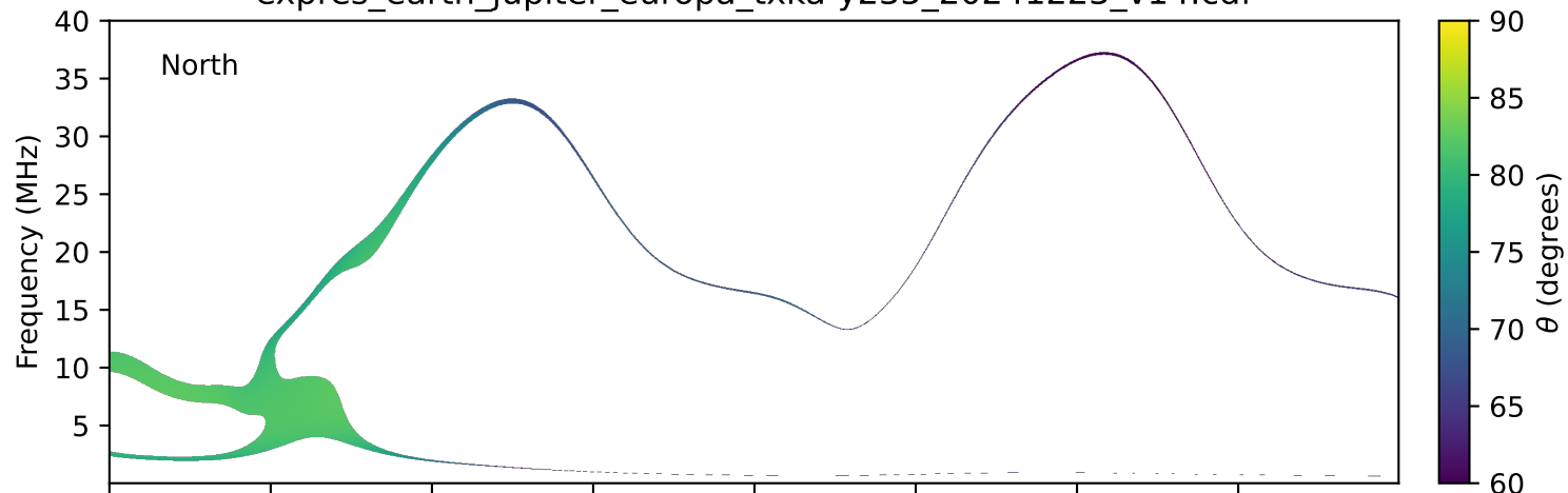
expres_earth_jupiter_europa_txka-y235_20241223_v14.cdf
