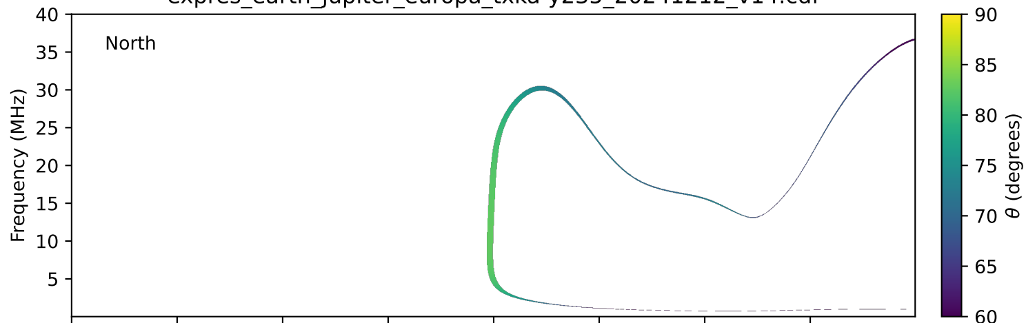
expres_earth_jupiter_europa_txka-y235_20241212_v14.cdf
