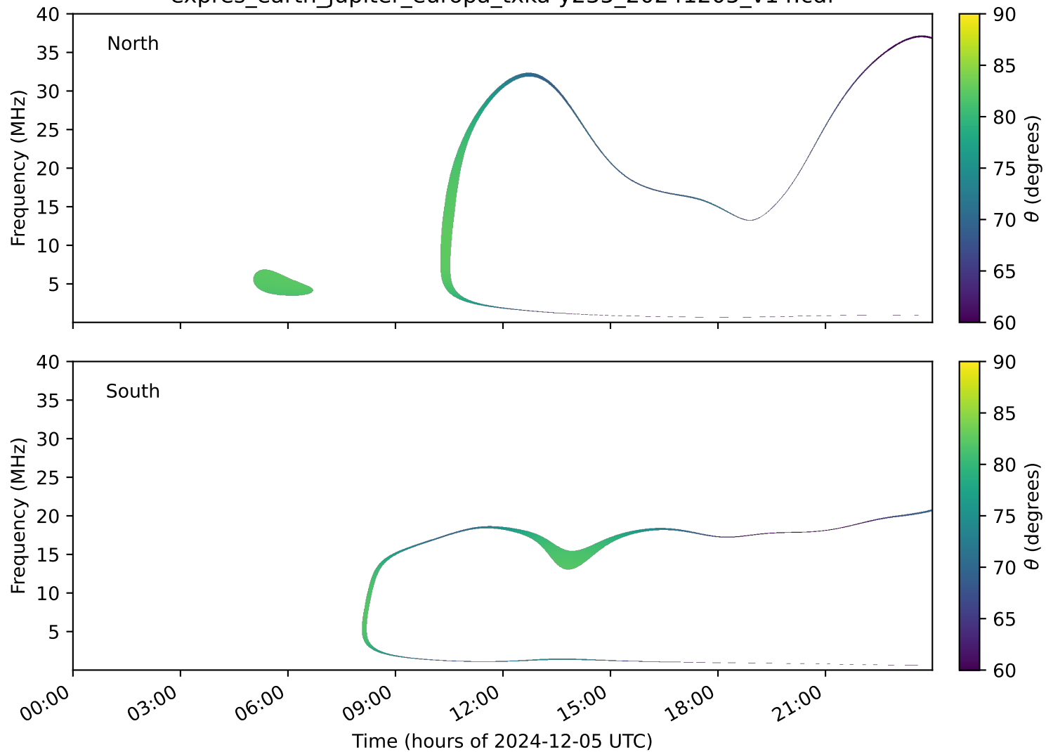
expres_earth_jupiter_europa_txka-y235_20241205_v14.cdf
