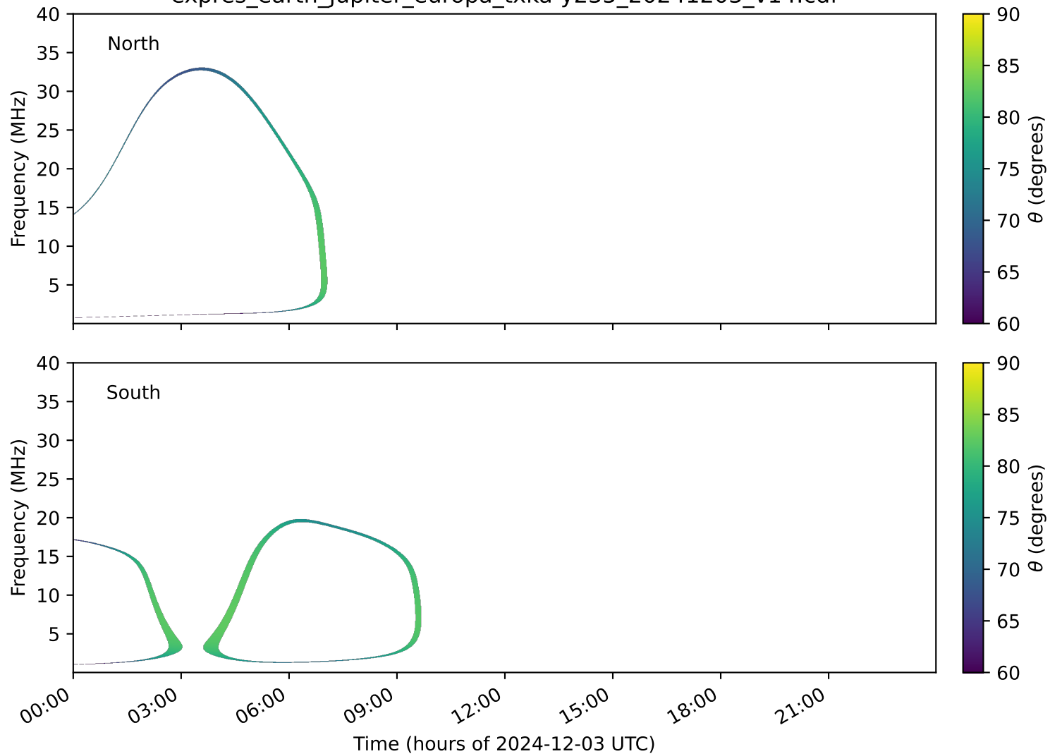
expres_earth_jupiter_europa_txka-y235_20241203_v14.cdf
