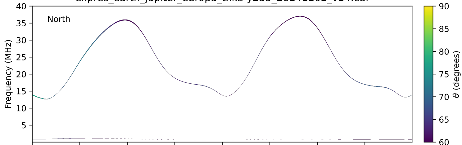
expres_earth_jupiter_europa_txka-y235_20241202_v14.cdf
